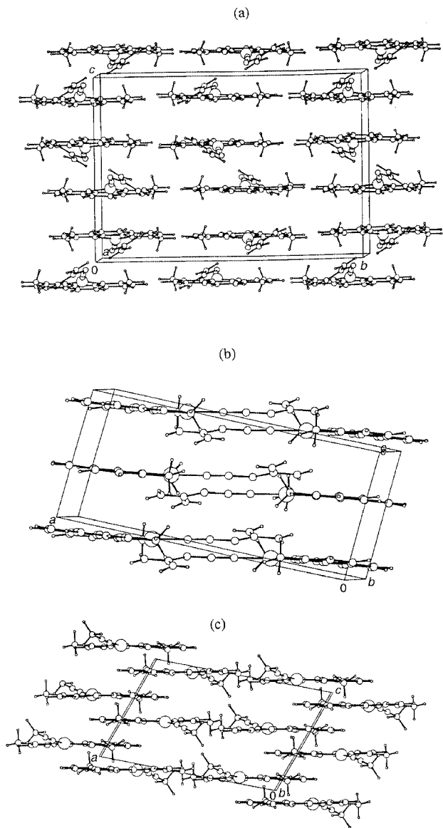
Fig. 3 Packing diagrams showing the parallel stacking of the cations of (a) [\text{Cu}(\text{dmp})(\text{cnge})][\text{BF}_4] \cdot 0.5\text{Et}_2\text{O} , (b) [\text{Cu}(\text{dmp})(\text{cnge})][\text{BF}_4] \cdot \text{MeCN} and (c) [\text{Cu}(\text{dmp})(\text{NCMe})][\text{BF}_4] .
