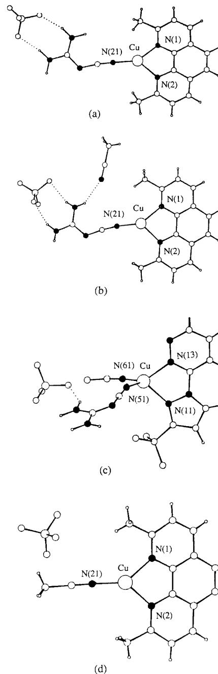
Fig. 1 The molecular structures of (a) [\text{Cu}(\text{dmp})(\text{cnge})][\text{BF}_4]\cdot 0.5\text{Et}_2\text{O} , (b) [\text{Cu}(\text{dmp})(\text{cnge})][\text{BF}_4]\cdot \text{MeCN} , (c) one of the terminal copper(I) centres in [\text{Cu}\{\mu\text{-ppdBu}\}\text{Cu}(\text{cnge})(\text{NCMe})][\text{BF}_4]\cdot \text{MeCN} and (d) [\text{Cu}(\text{dmp})(\text{NCMe})][\text{BF}_4] depicting the associative substitution of 2-cyanoguanidine by acetonitrile at trigonal planar copper(I). [In the ligands, open circles represent carbon atoms and filled circles nitrogen atoms.]
