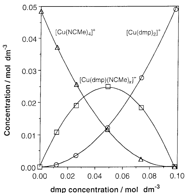
Fig. 6 Variation in the composition of acetonitrile solutions containing copper(I) tetrafluoroborate ( 0.0485 \text{ mol dm}^{-3} ) and 2,9-dimethyl-1,10-phenanthroline ( 0.00 – 0.0970 \text{ mol dm}^{-3} ) at 298 K.
